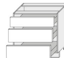
D3M 80 ● (800/820/500)
