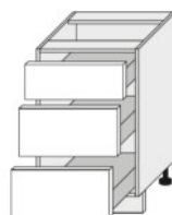
D3M 50 ● (500/820/500)
