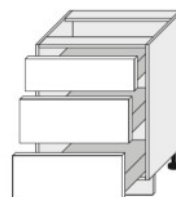
D3M 60 ● (600/820/500)
