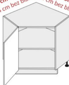
D12R 90 L/P (840/820/840)
