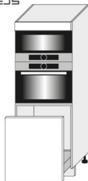
D5AR 60 / 154 (600/1540/565)
