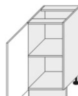
D1D 40 L/P (400/820/500)
