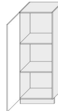
D5D 60 / 154 L (600/1540/565)
