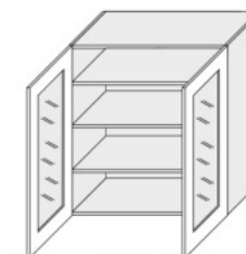
W4S 90 (900/960/325)
