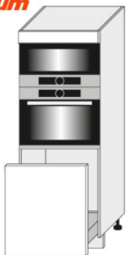
D5AM 60 / 154 ● (600/1540/565)
