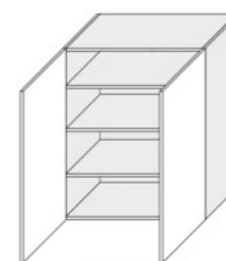
W4 80 (800/960/325)
