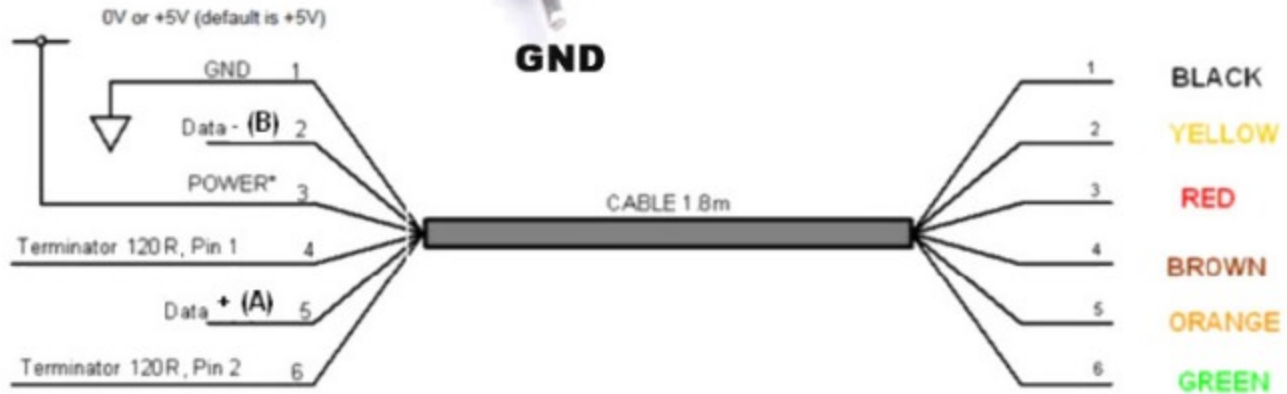
USB-RS485-WE Connections
