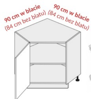
D12R 90 (840/820/840)
