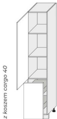
2D14K 40 L/P (400/2070/565)
